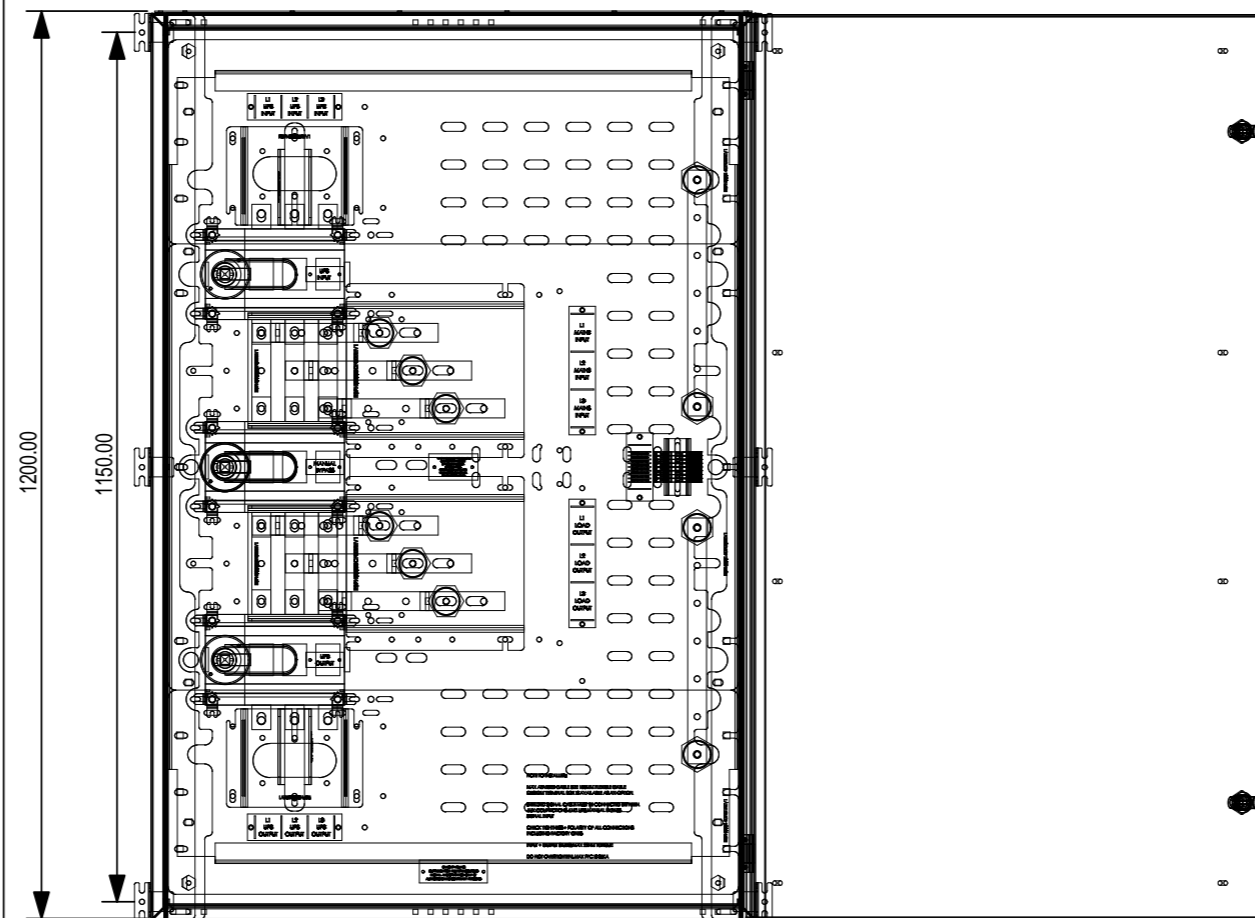
FRONT VIEW:
